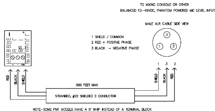
Figure 1. Cable connections
