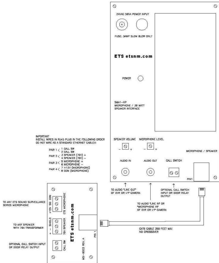
CONNECTIONS TO MSI-BOC5 (SEPARATE MICROPHONE AND SPEAKER)
