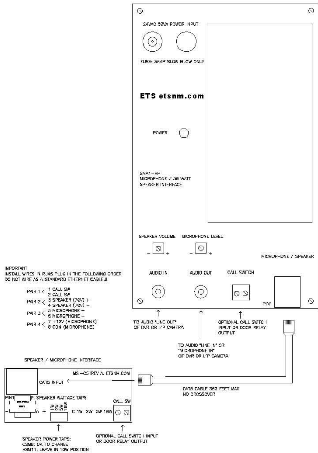
CONNECTIONS TO MSI-C5 (HSM11)
