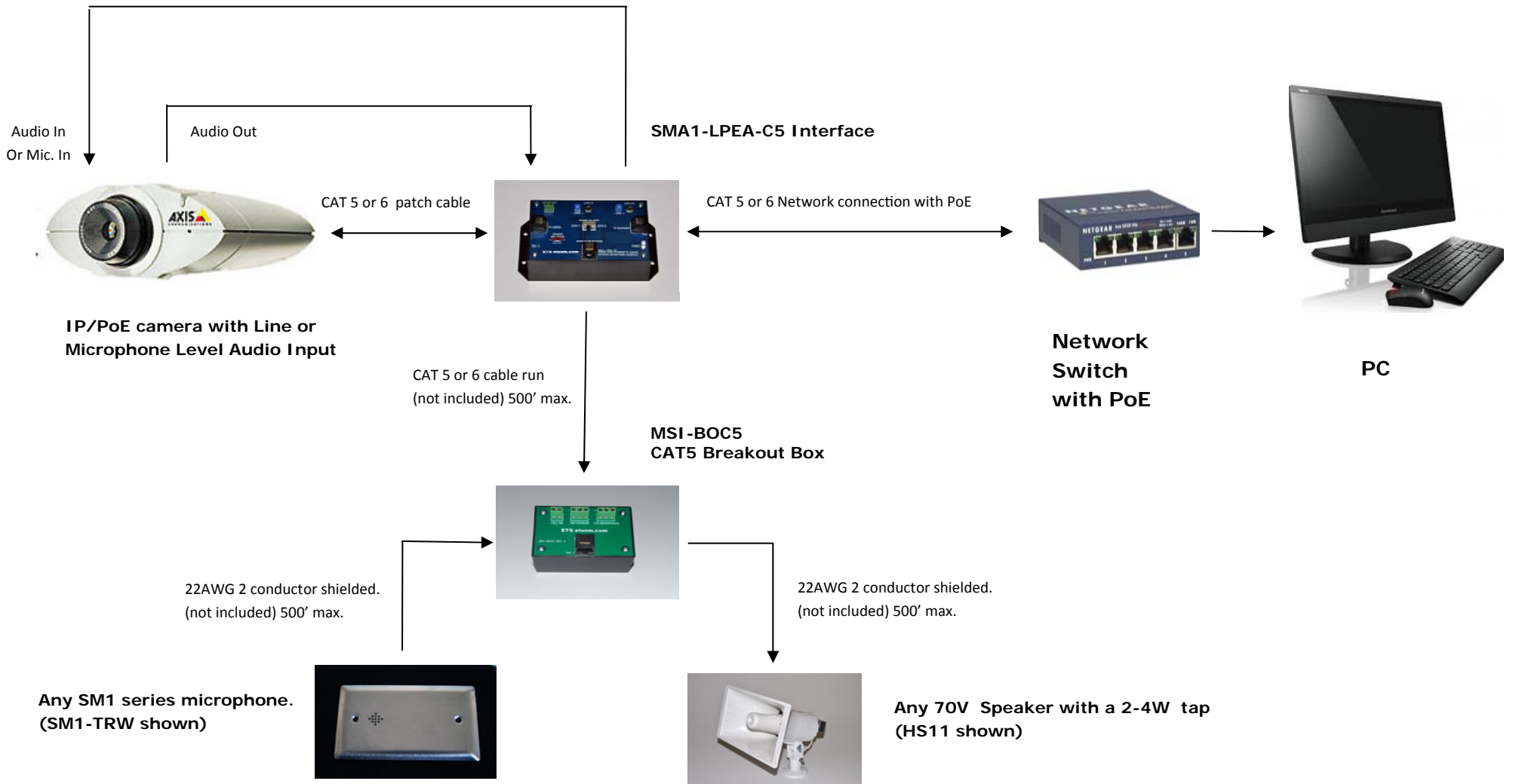
Application Diagram 2 of 2 SMA1-LPEA-C5 with MSI-BOC5
