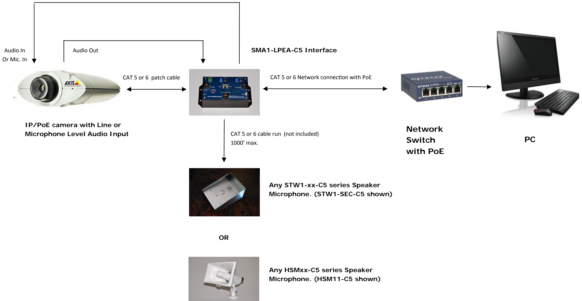
Application Diagram 1 of 2 SMA1-LPEA-C5
