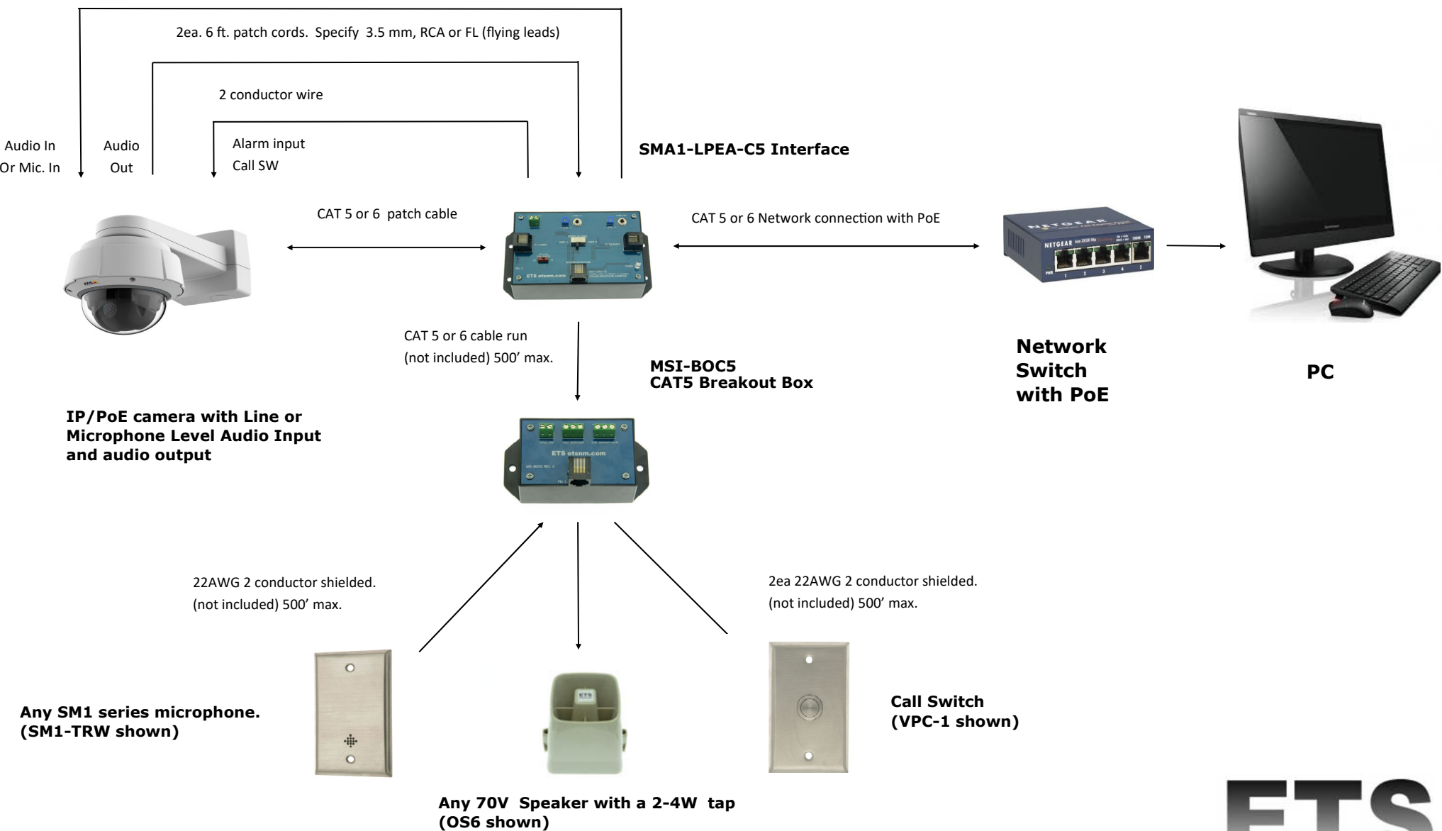
Application Diagram 2 of 2 SMA1-LPEA-C5 with MSI-BOC5
