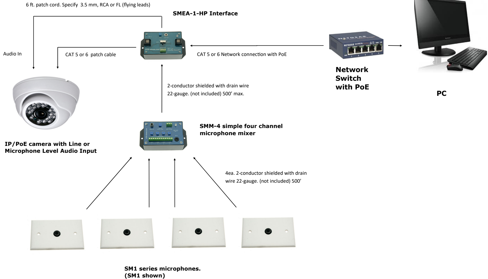
Application Diagram 1 of 2 SMEA-1-HP with SMM4 zone expansion
